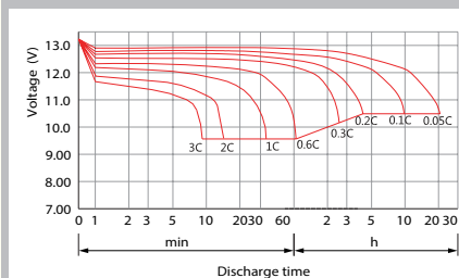
Discharge Characteristics (25°C)
